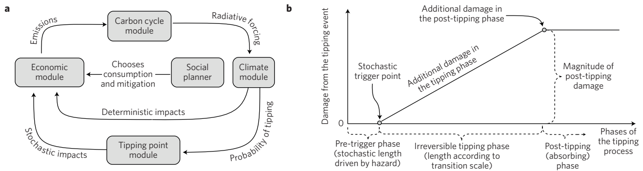
Figure 1 | Schematic of the DSICE model. a , The forward-looking decision-maker (social planner) chooses mitigation and consumption to maximize the sum of discounted expected utilities over some time horizon. Increased mitigation must be traded off against consumption and savings. Global warming adversely impacts the economy and increases the probability of a tipping point with additional irreversible economic impacts. b , The length of the pre-tipping phase is stochastic, and its likelihood depends on global warming. Once tipping is triggered, damages increase linearly over a specified transition time (5–500 years here) to a specified final level (2.5–20% of World GDP here).
