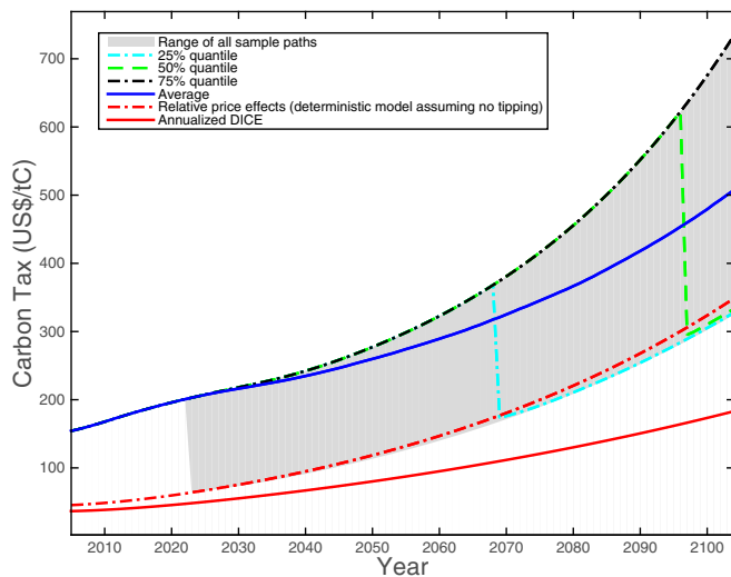
Fig. 3. The optimal carbon taxes (in US dollars per metric ton of carbon) for the case in which the tipping point impacts market and nonmarket goods: \sigma=0.5 , \gamma=0.02 , P^*=5\% , J_S^*=5\% , and J_Y^*=5\% (see Approach for parameter definitions). The state of the environmental good crosses a tipping point probabilistically, and so the paths of 25%, 50%, and 75% quantiles and of the average are shown as well as the range of all sample paths and two reference paths (the path of the annualized DICE model and the path with relative price effects from the deterministic model assuming no tipping).
