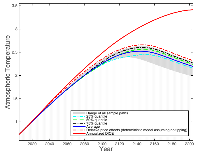
Fig. 2. The increases of the global surface temperature from the preindustrial time for the case in which the tipping point only impacts nonmarket goods. The paths of quantiles and the average are shown as well as the range of all sample paths and two reference paths (the path of the annualized DICE model and the path with relative price effects from the deterministic model assuming no tipping).
