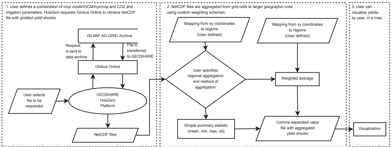
Fig. 1. AgMIP tool workflow.
